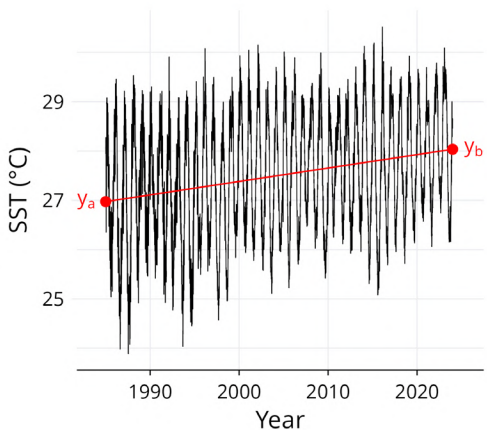
Figure 3.2. Illustration of the linear regression performed on the SST time-series, and the points ( y_a = first point of the long-term trend, y_b = last point of the long-term trend) used to estimate the average change in SST and the average annual warming rate. The data used in this example are from Fijian coral reefs.
