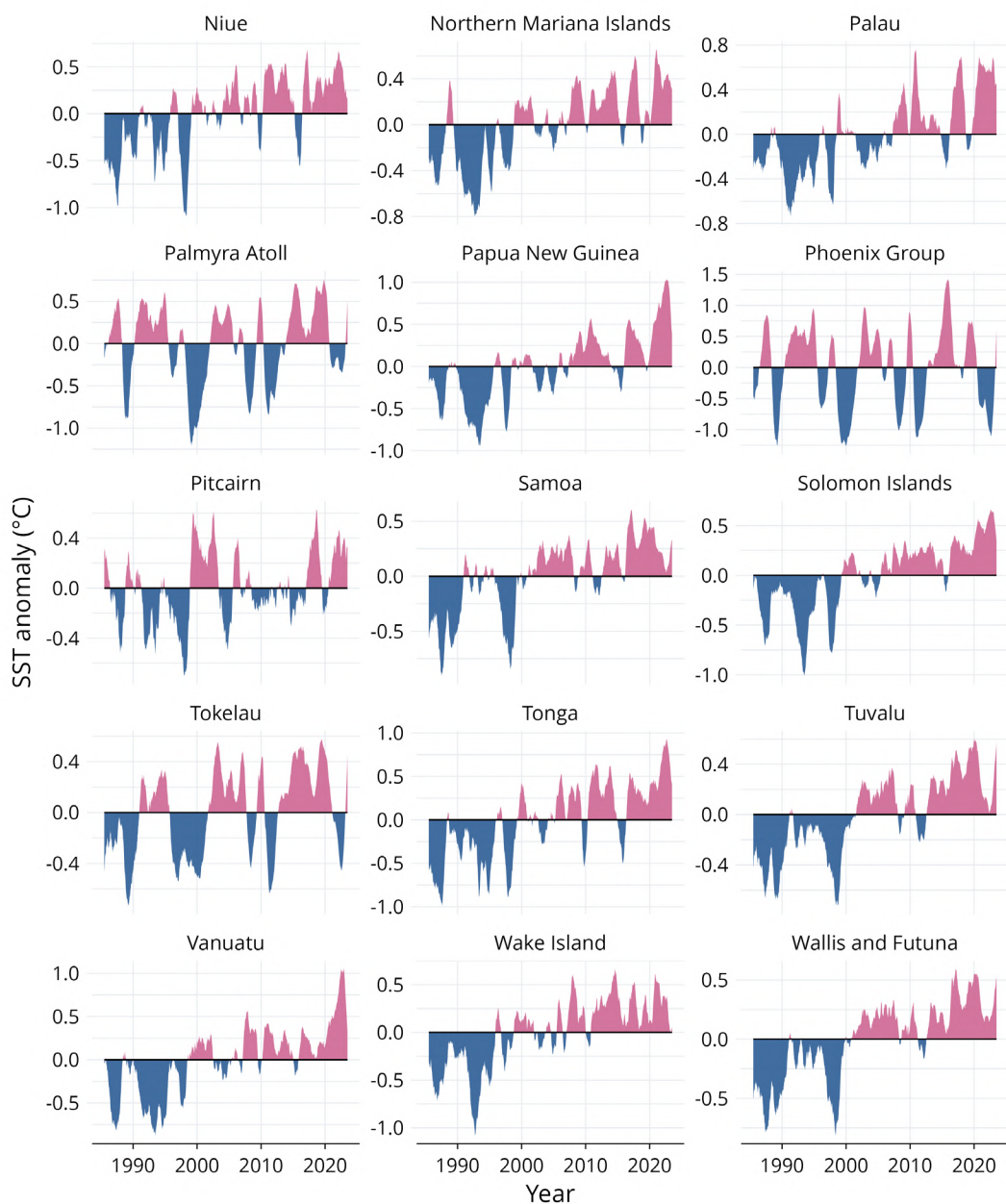
▲ Supplementary Figure 3 (continuing). Average Sea Surface Temperature (SST) anomaly from 1985 to 2023 over coral reefs of countries and territories of the Pacific. The black line represents a null SST anomaly; values below this line are negative SST anomalies ( i.e. , cooler than the long-term average), and values above this line are positive SST anomalies ( i.e. , warmer than the long-term average).
